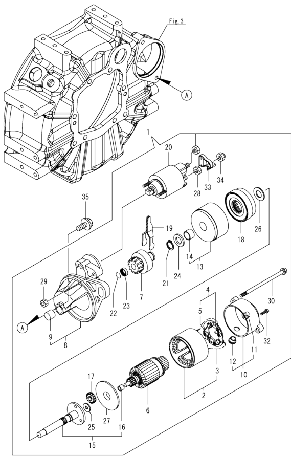
Fig.14. STARTER MOTOR
