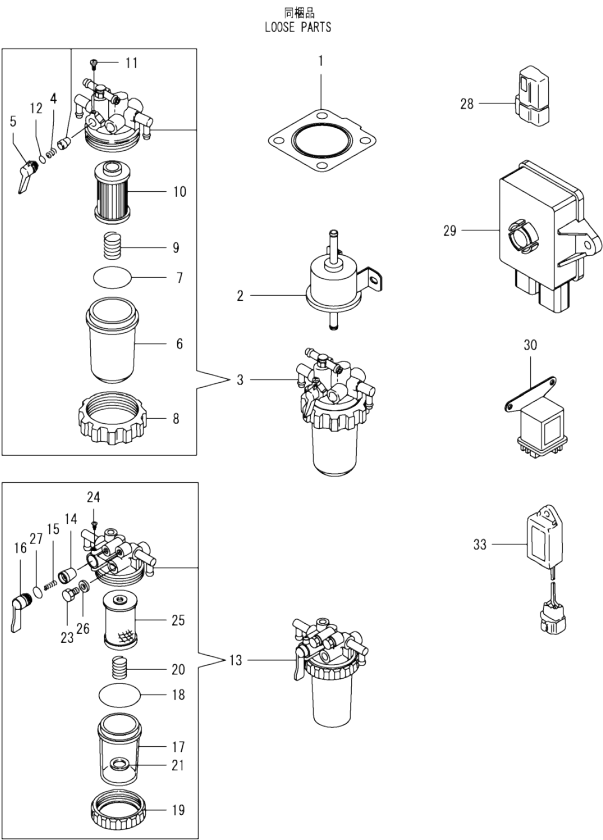
Fig.16. ACCESSORY
