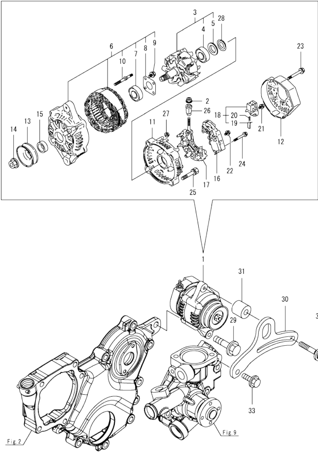
OCD50-M02320 ENGINE Fig.15. GENERATOR
